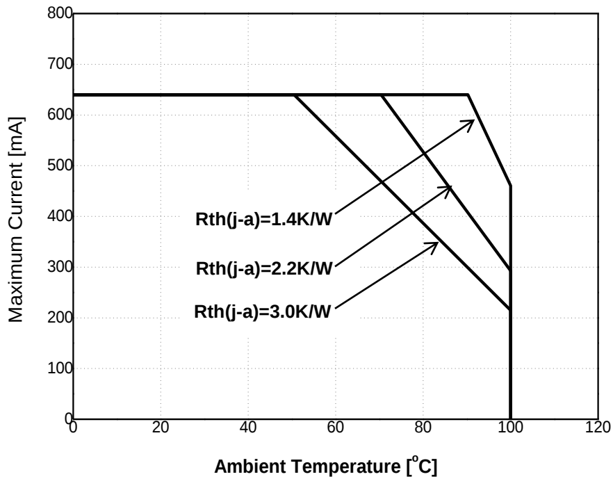
Fig 9. Maximum Forward Current vs. Ambient Temperature, T_j(\text{max.}) = 125^\circ\text{C} , I_F = 0.64\text{A}
