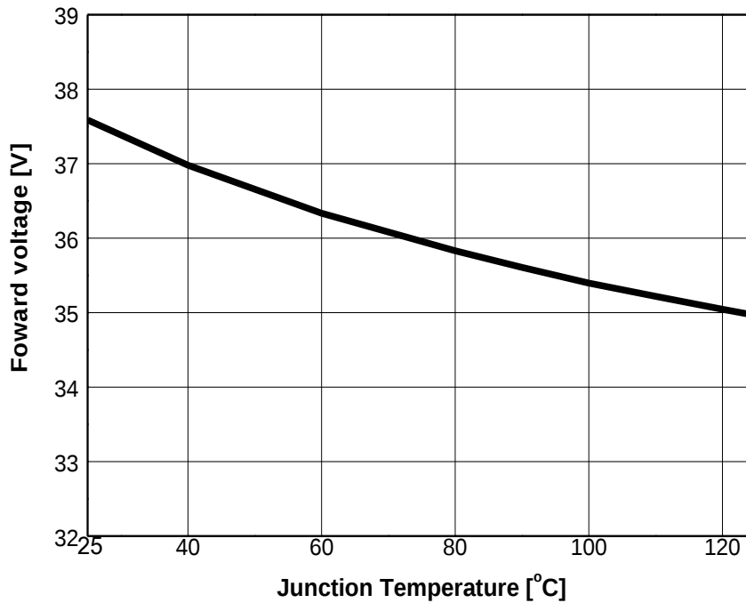
Fig 8. Forward Voltage vs. Junction Temperature, I_F = 500\text{mA}
