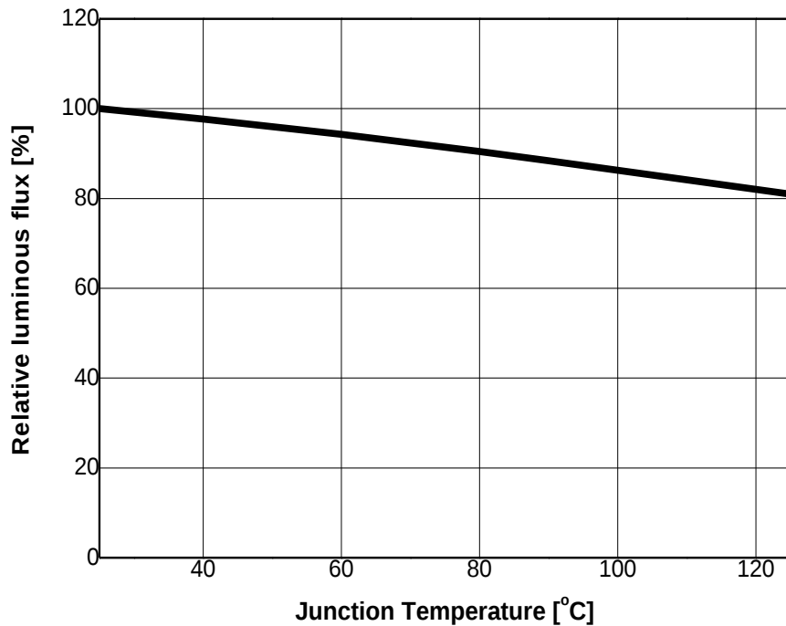
Fig 6. Relative Light Output vs. Junction Temperature, I_F = 500\text{mA}
