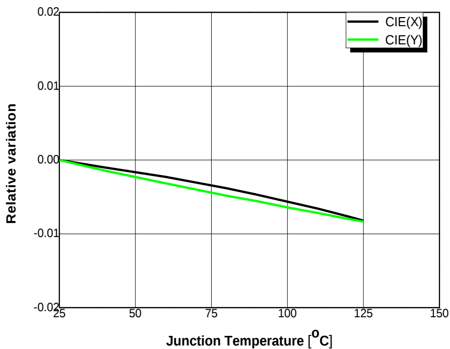
Fig 7. Junction Temp. vs. CIE X, Y Shift, I_F = 500\text{mA} (Warm white)
