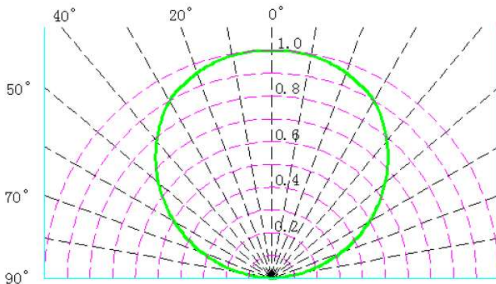
Curves of beam angel and relative brightness 角度图
